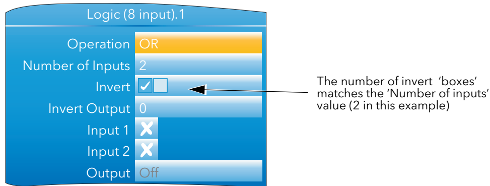
Figure 4.21 Eight input logic block configuration
