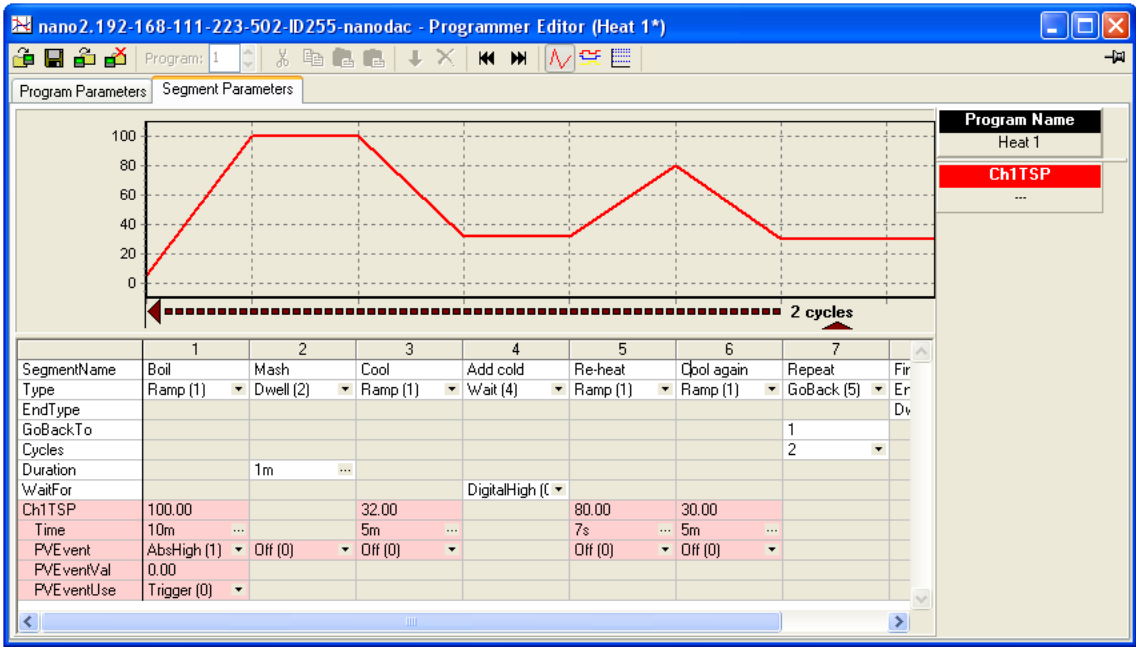
Figure 6.6 Programmer display
