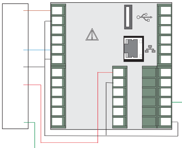
Figure 3.4.9m BCD Switch Physical Wiring
