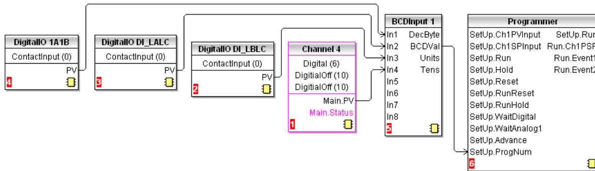
Figure 3.4.9l BCD Switch Wiring
