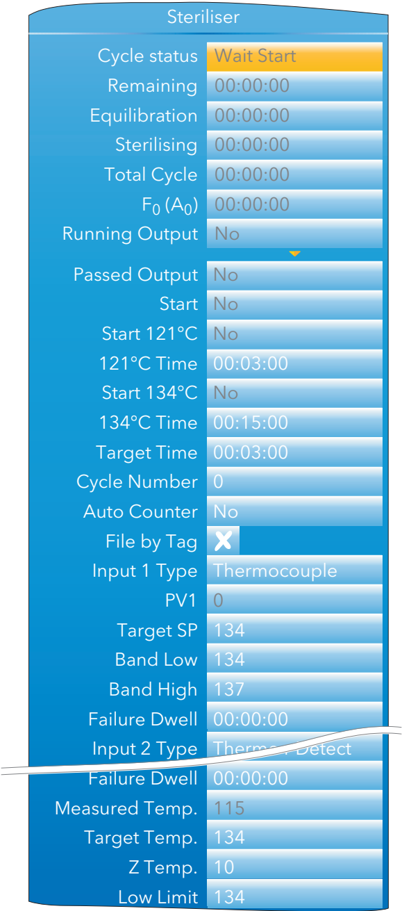
Figure 4.17 Steriliser block configuration menu
