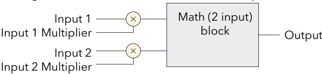
Figure 4.23a Block schematic
