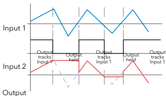
Figure 4.23.2 Sample and Hold example
