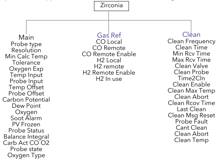
Figure 4.16.2a Zirconia probe configuration layout.
