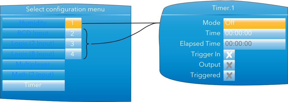
Timer block (Section 4.23)
