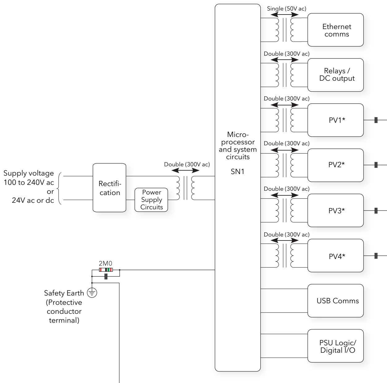
Figure C5 Isolation diagram
