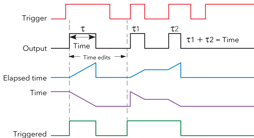
Figure 4.24.2c 'One Shot' timer definitions
