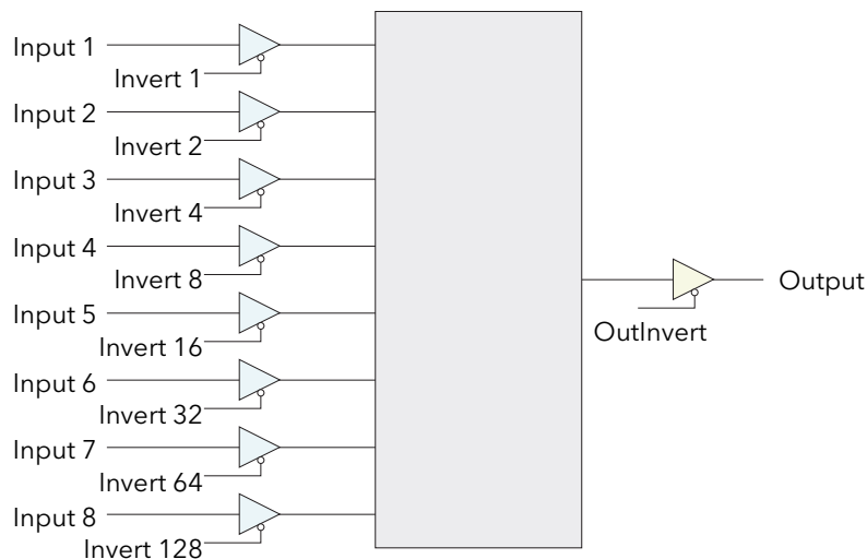
Figure 4.21.2 Logic (8 input) block schematic
